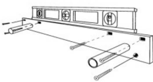
OPTION 2 - MOUNTING BAR
